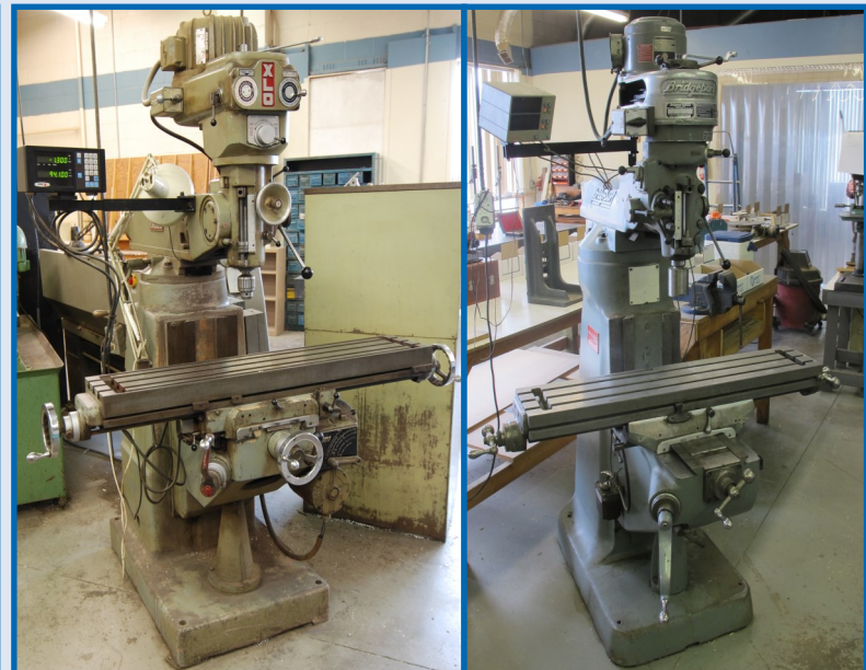
BRIDGEPORT & EX-CELL-O VERTICAL MILLING MACHINES
